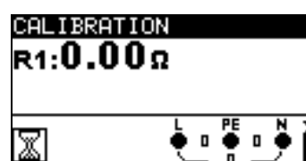
Reading at calibrated value is 0.00 \Omega now.
