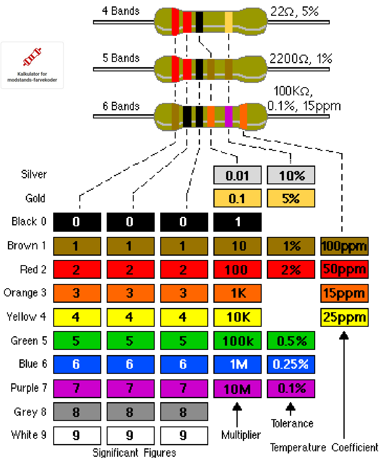
Resistor Color Code System
