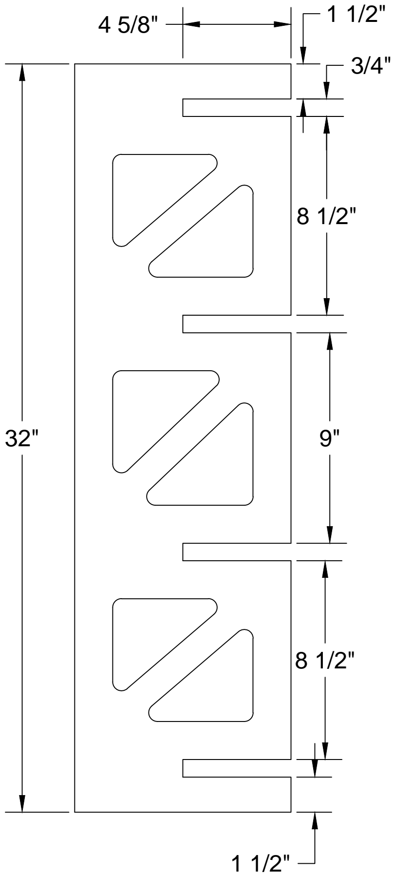
2x Sides from 1x10 board
