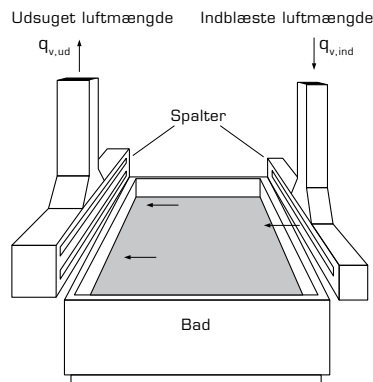
Figur 6.5. Push-pull system.
